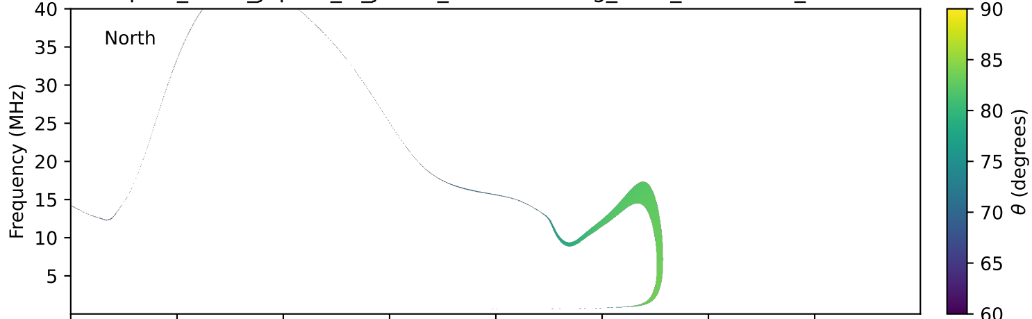
expres_earth_jupiter_io_jrm09_lossc-wid1deg_3kev_19980807_v11.cdf
