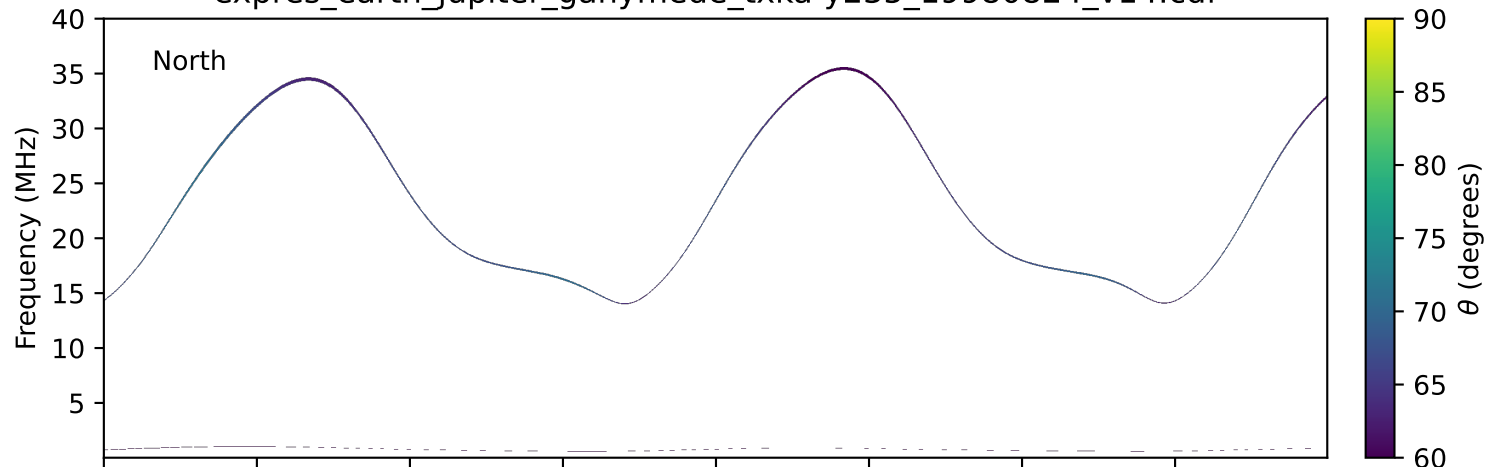
expres_earth_jupiter_ganymede_txka-y235_19980824_v14.cdf
