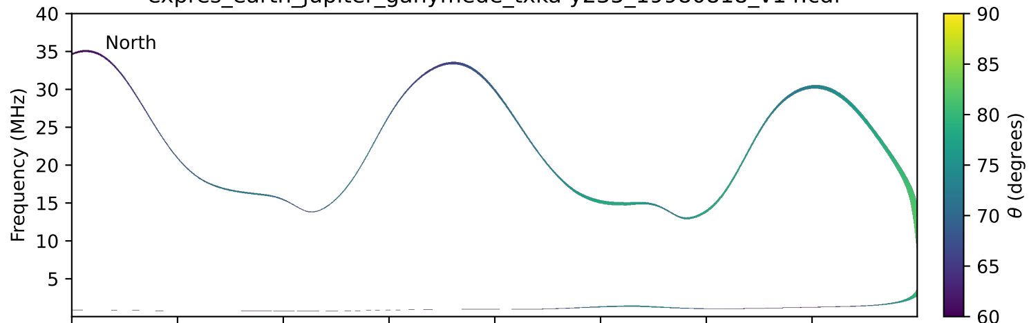
expres_earth_jupiter_ganymede_txka-y235_19980818_v14.cdf
