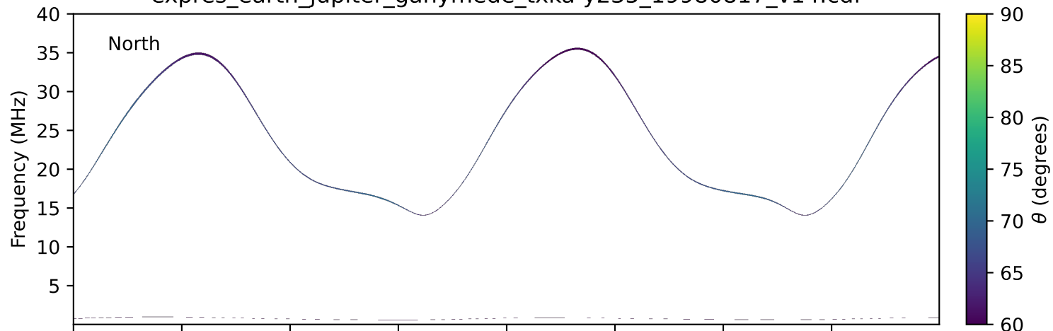
expres_earth_jupiter_ganymede_txka-y235_19980817_v14.cdf
