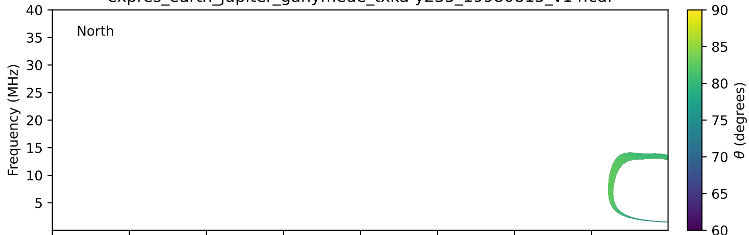
expres_earth_jupiter_ganymede_txka-y235_19980815_v14.cdf
