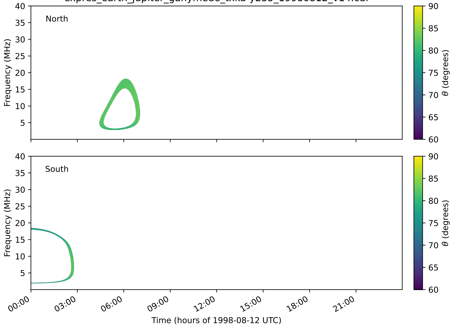
expres_earth_jupiter_ganymede_txka-y235_19980812_v14.cdf
