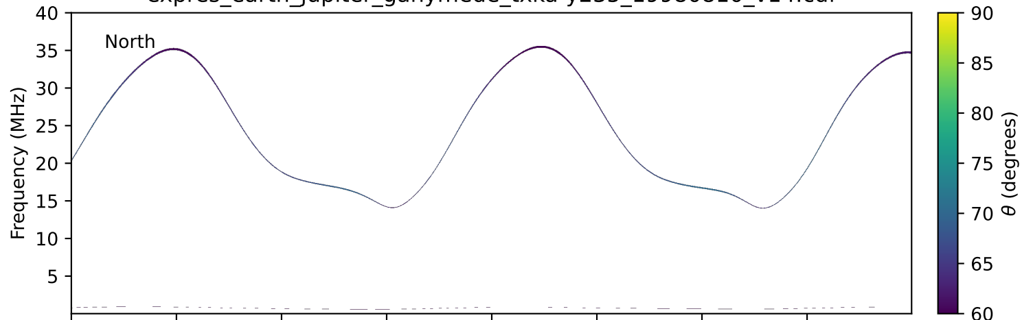
expres_earth_jupiter_ganymede_txka-y235_19980810_v14.cdf
