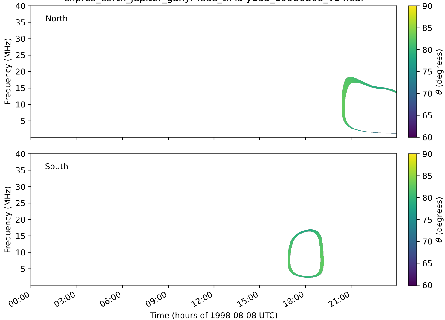
expres_earth_jupiter_ganymede_txka-y235_19980808_v14.cdf
