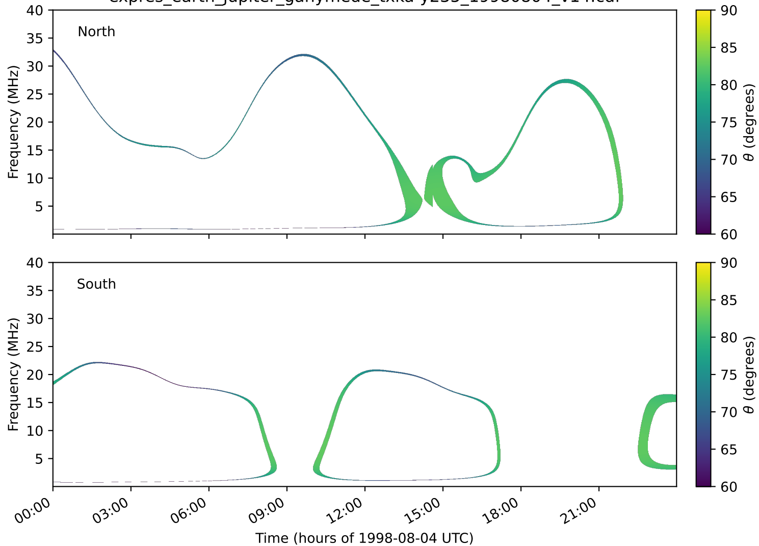
expres_earth_jupiter_ganymede_txka-y235_19980804_v14.cdf
