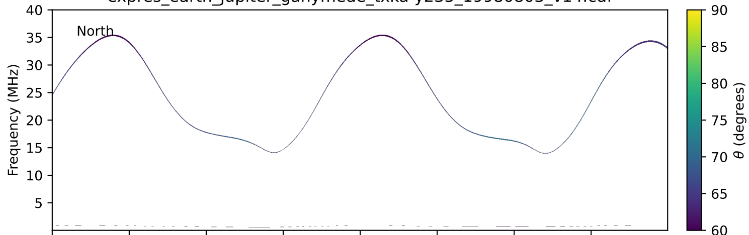
expres_earth_jupiter_ganymede_txka-y235_19980803_v14.cdf
