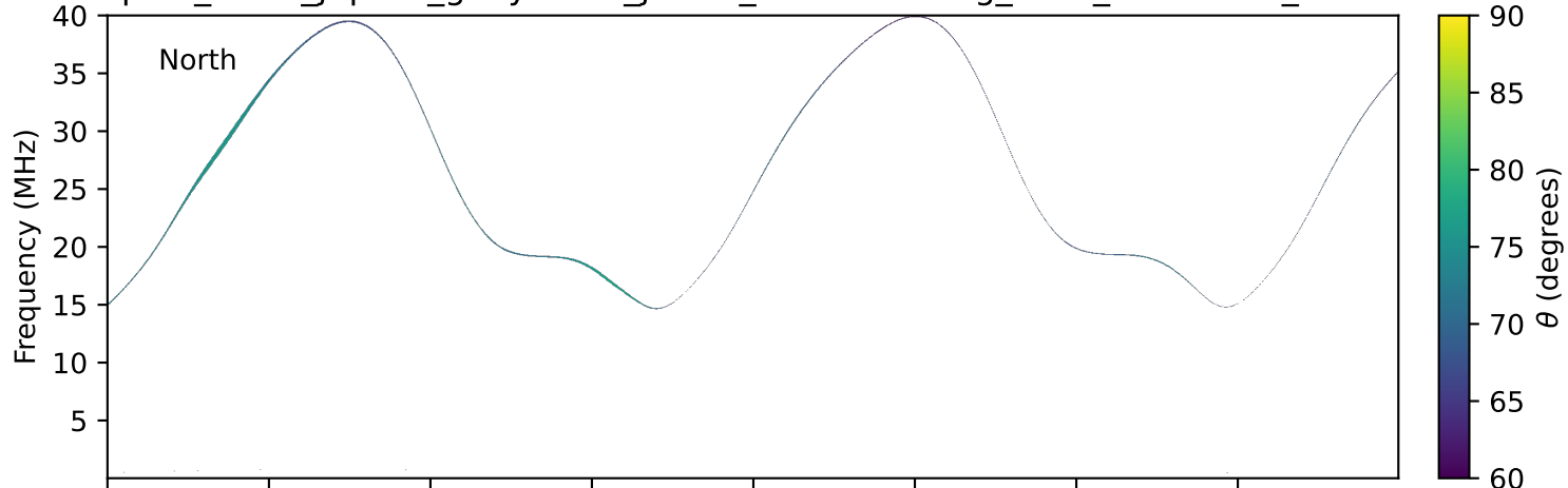
expres_earth_jupiter_ganymede_jrm33_lossc-wid1deg_3kev_19980831_v11.cdf
