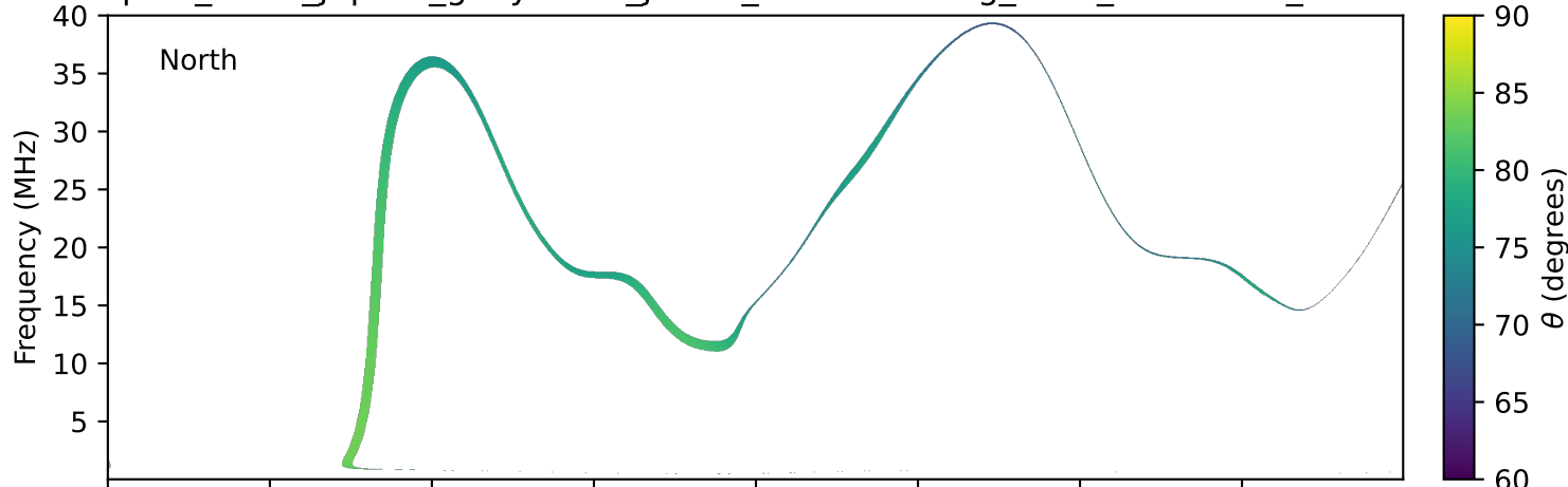
expres_earth_jupiter_ganymede_jrm33_lossc-wid1deg_3kev_19980809_v11.cdf
