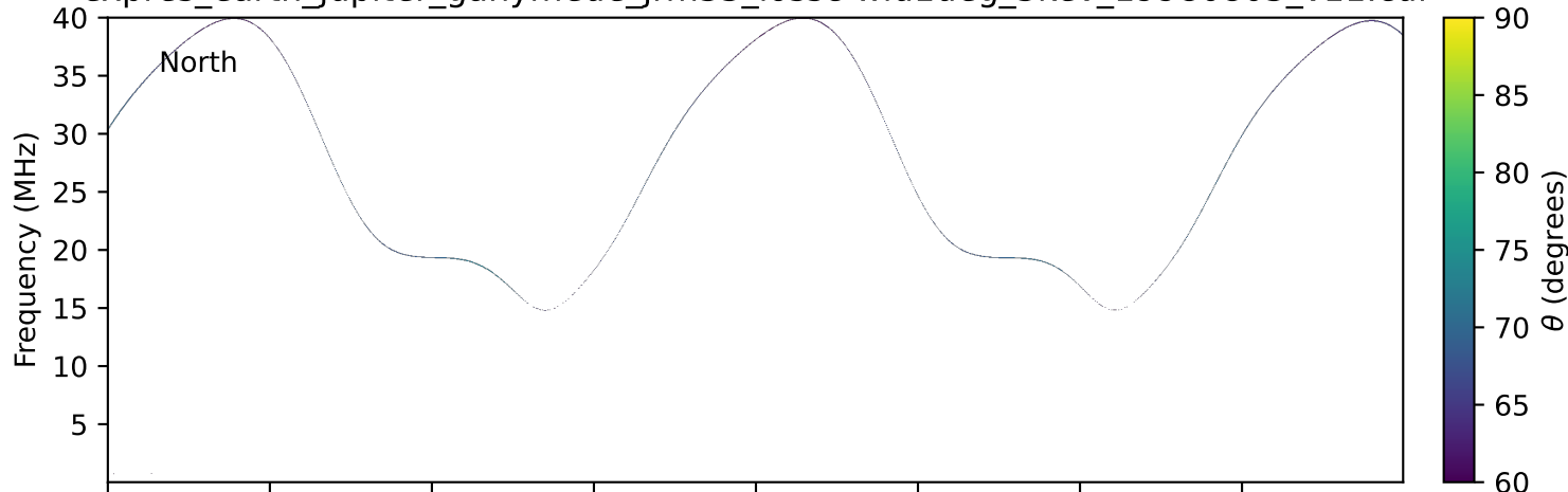
expres_earth_jupiter_ganymede_jrm33_lossc-wid1deg_3kev_19980803_v11.cdf
