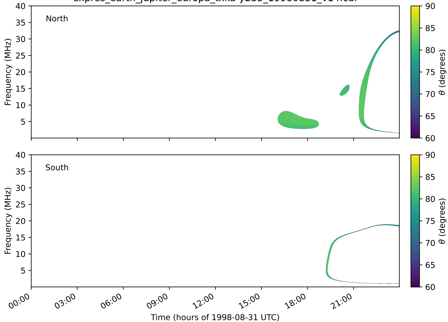
expres_earth_jupiter_europa_txka-y235_19980831_v14.cdf
