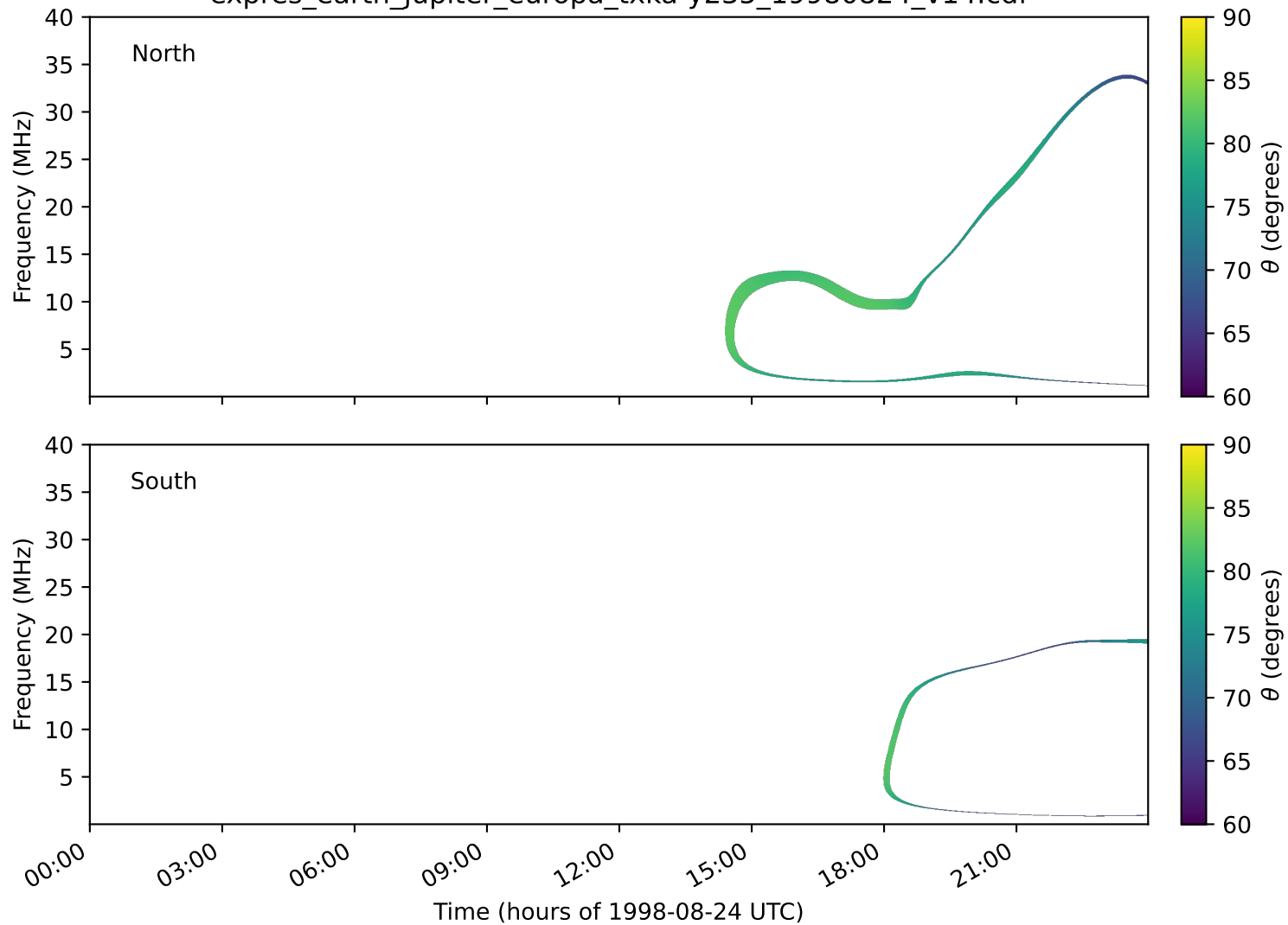
expres_earth_jupiter_europa_txka-y235_19980824_v14.cdf
