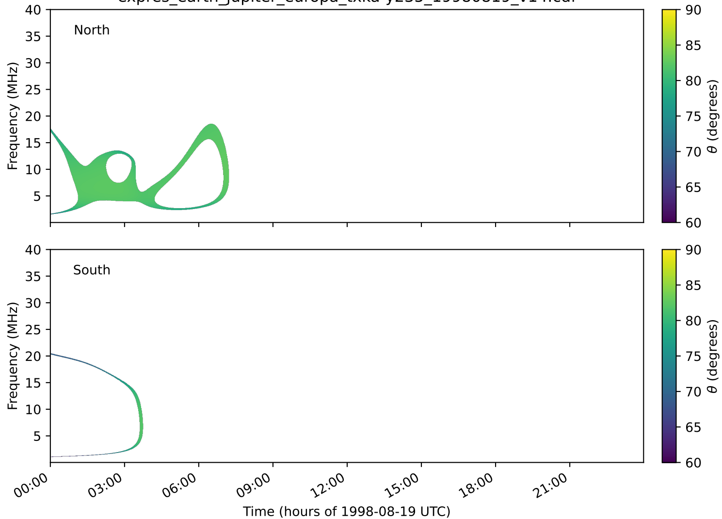
expres_earth_jupiter_europa_txka-y235_19980819_v14.cdf
