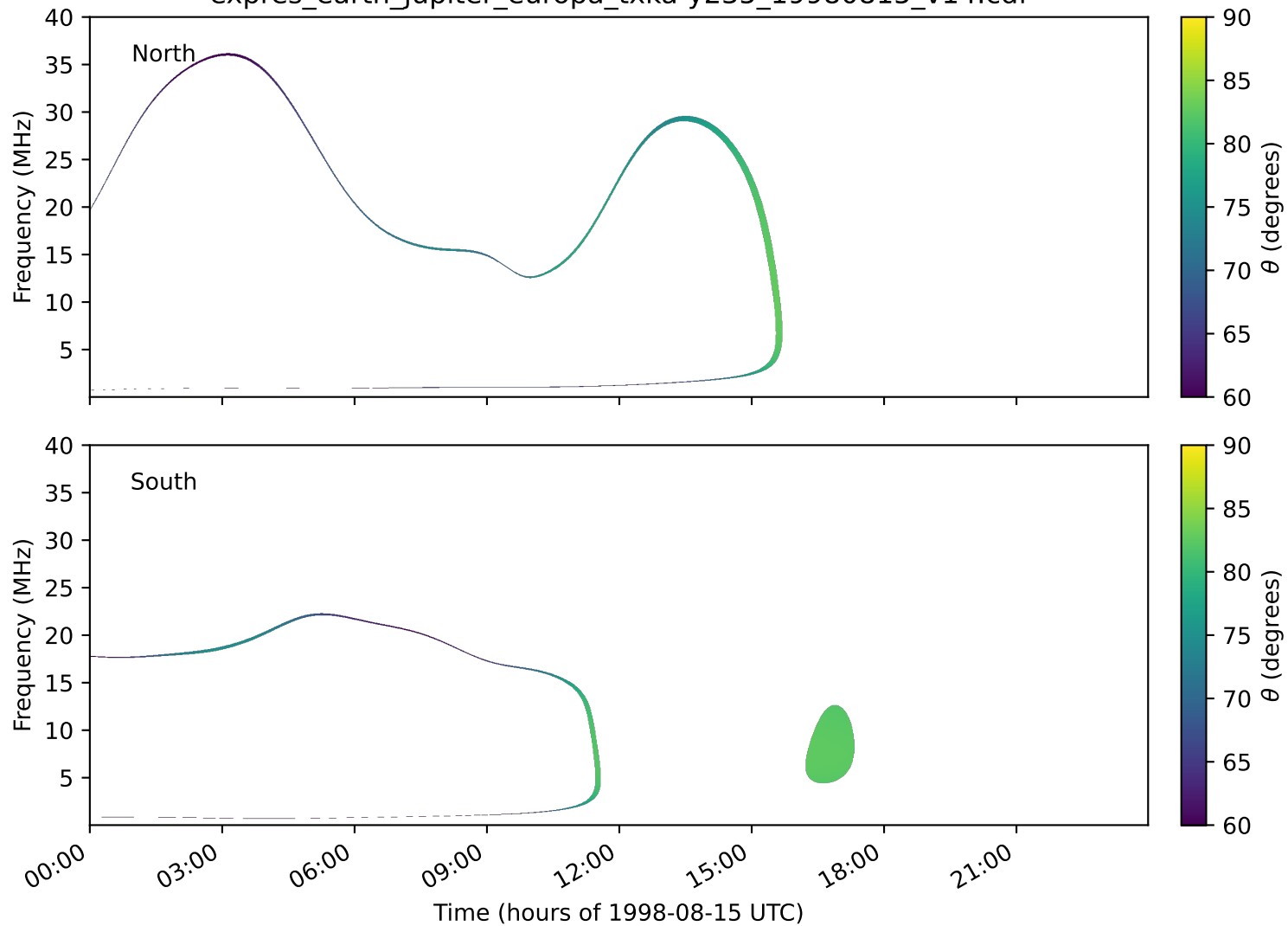
expres_earth_jupiter_europa_txka-y235_19980815_v14.cdf
