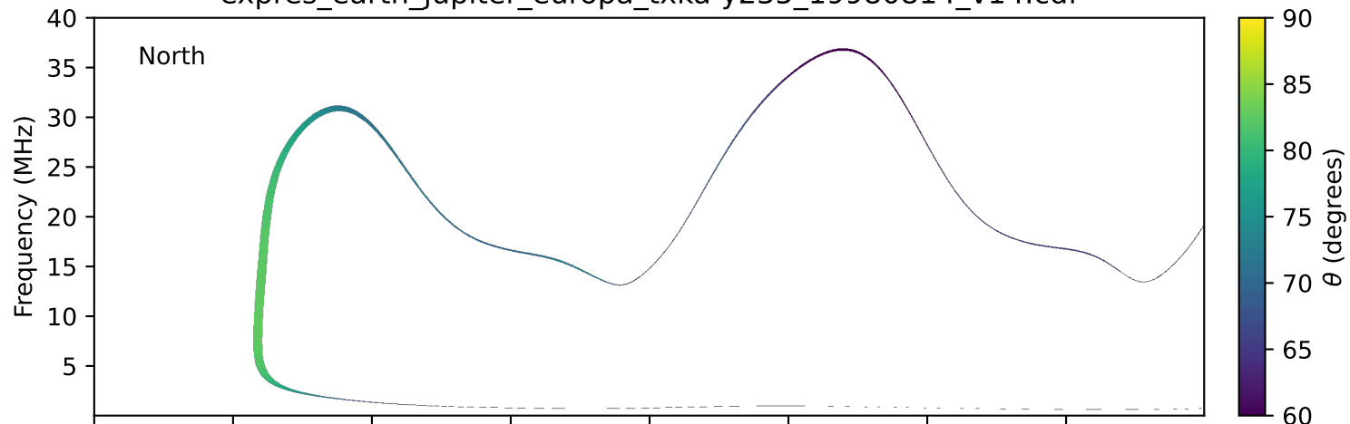
expres_earth_jupiter_europa_txka-y235_19980814_v14.cdf
