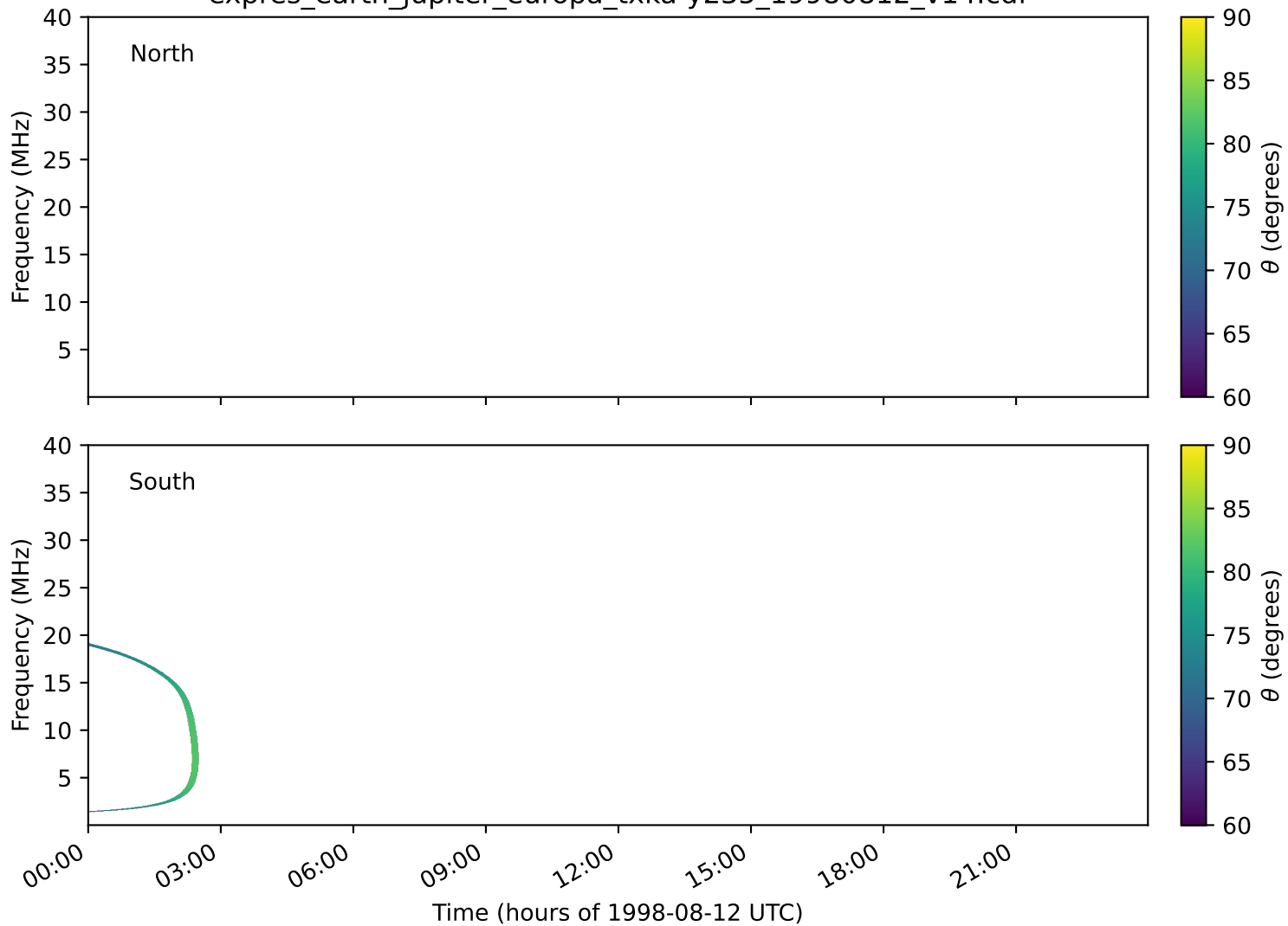
expres_earth_jupiter_europa_txka-y235_19980812_v14.cdf
