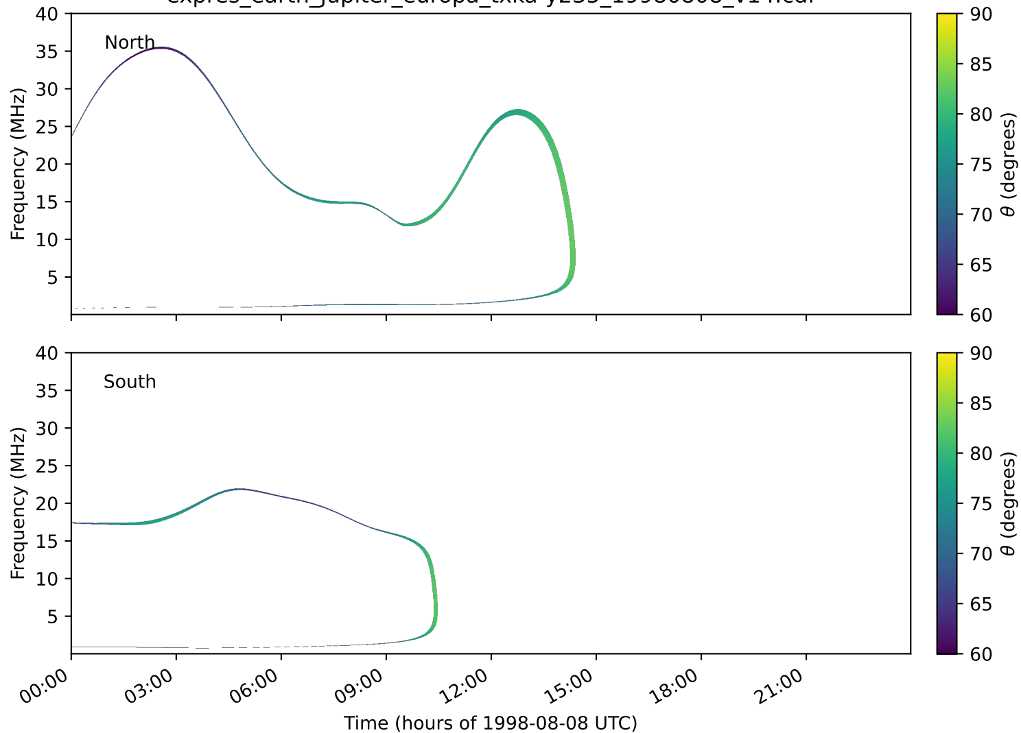
expres_earth_jupiter_europa_txka-y235_19980808_v14.cdf
