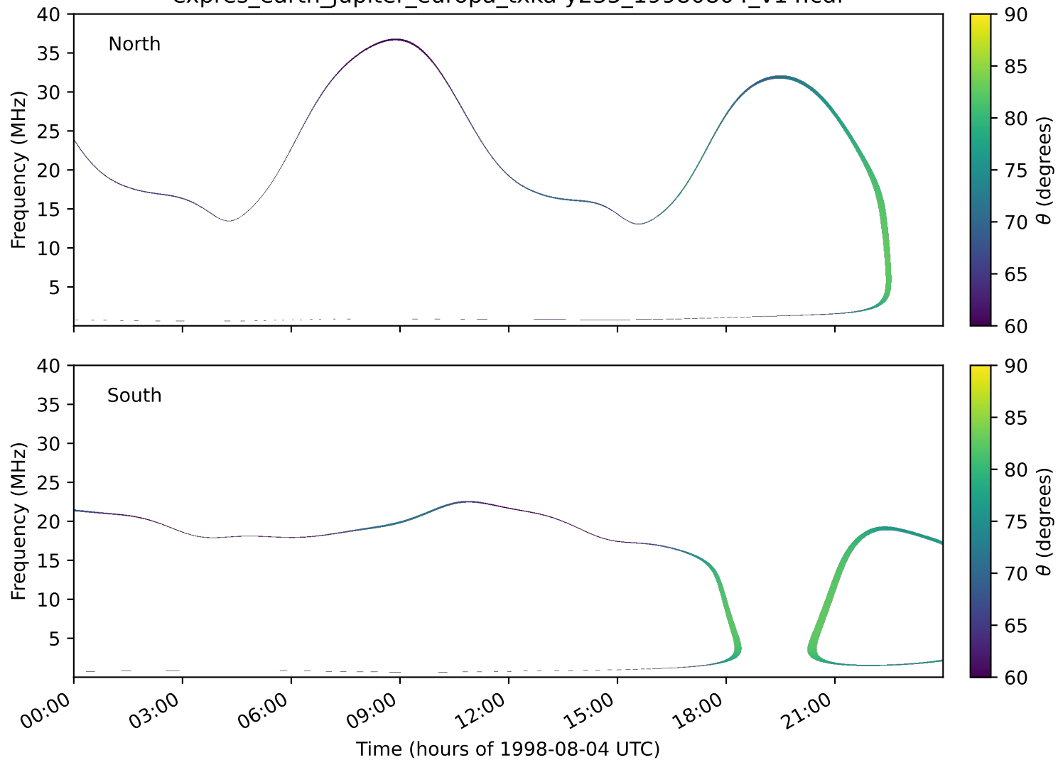
expres_earth_jupiter_europa_txka-y235_19980804_v14.cdf
