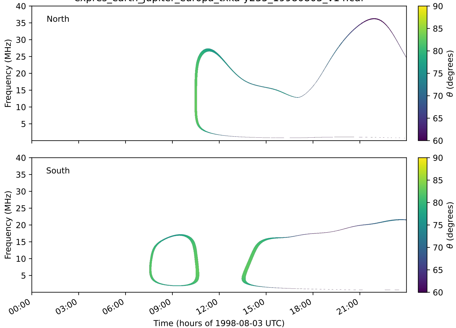
expres_earth_jupiter_europa_txka-y235_19980803_v14.cdf
