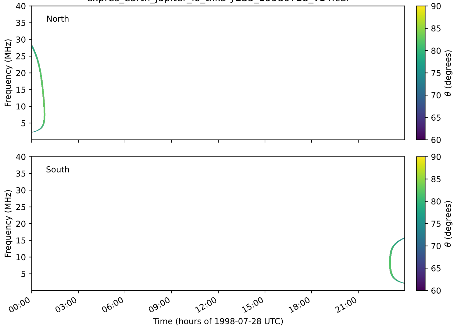
expres_earth_jupiter_io_txka-y235_19980728_v14.cdf
