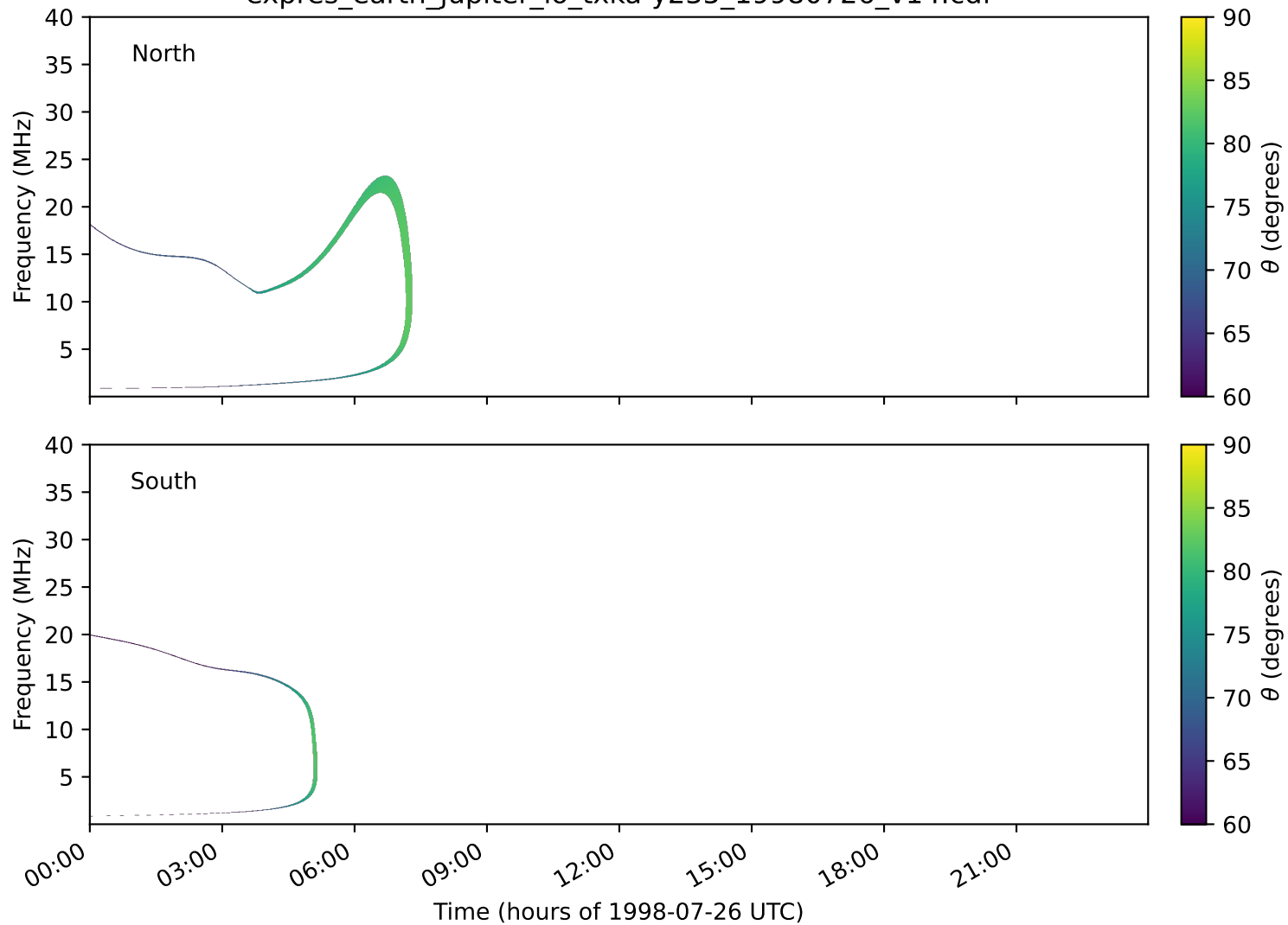
expres_earth_jupiter_io_txka-y235_19980726_v14.cdf
