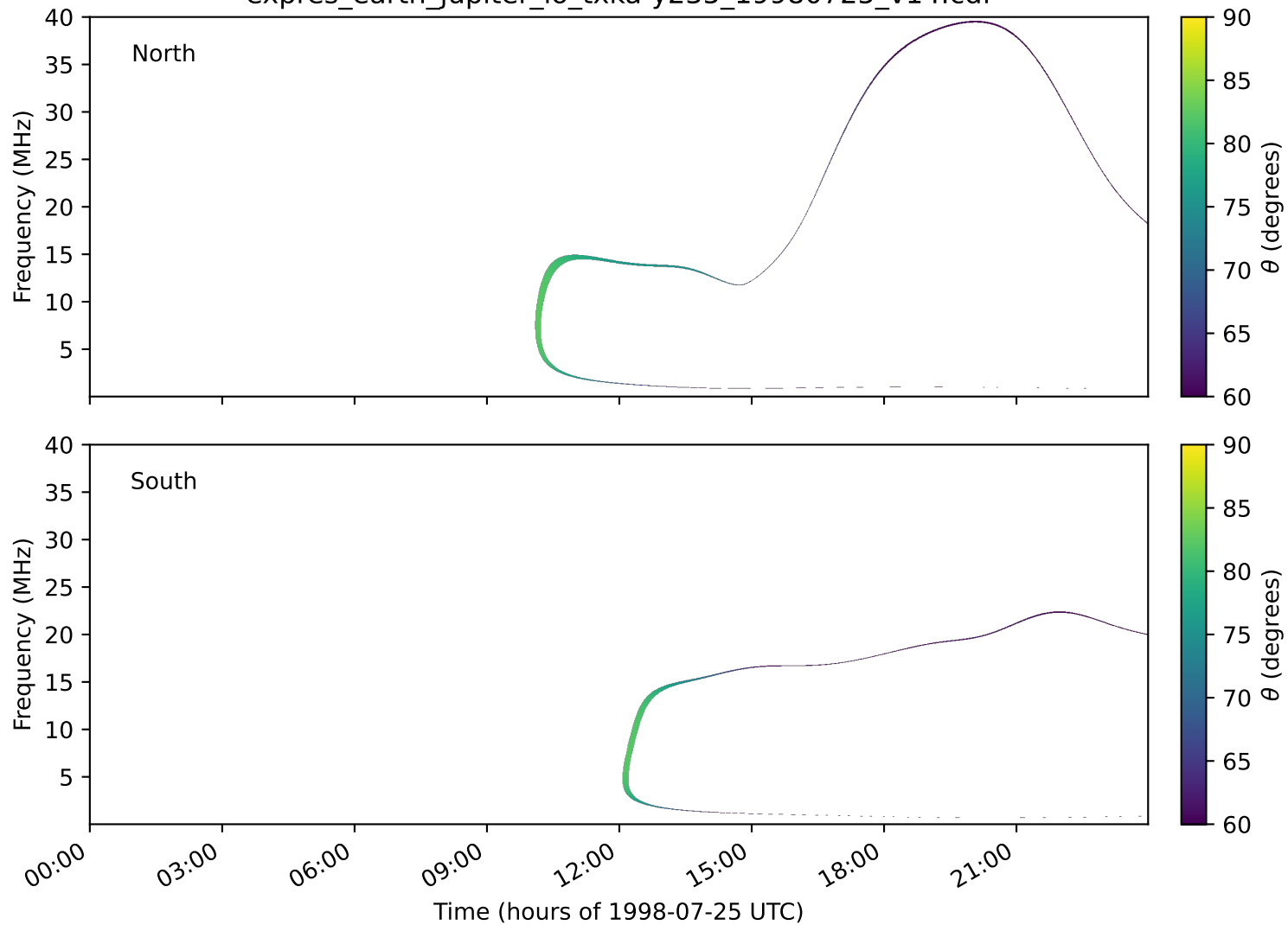
expres_earth_jupiter_io_txka-y235_19980725_v14.cdf
