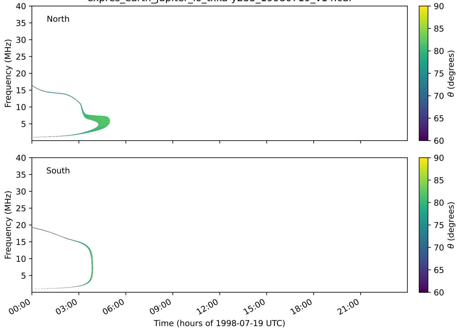
expres_earth_jupiter_io_txka-y235_19980719_v14.cdf
