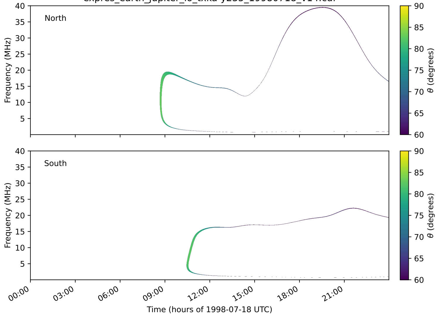
expres_earth_jupiter_io_txka-y235_19980718_v14.cdf
