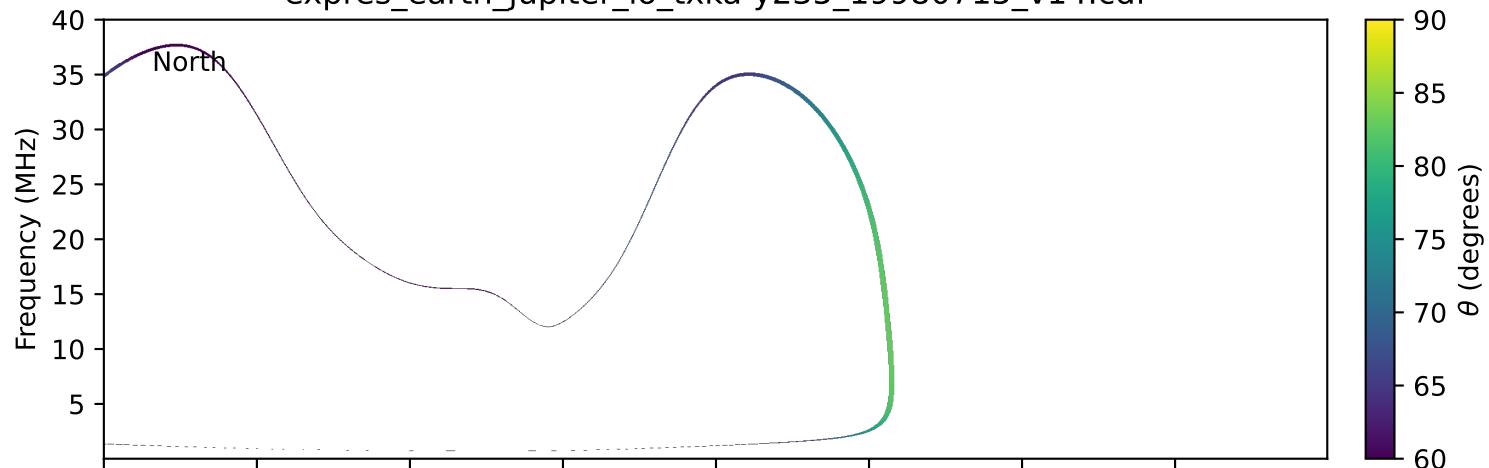
expres_earth_jupiter_io_txka-y235_19980715_v14.cdf
