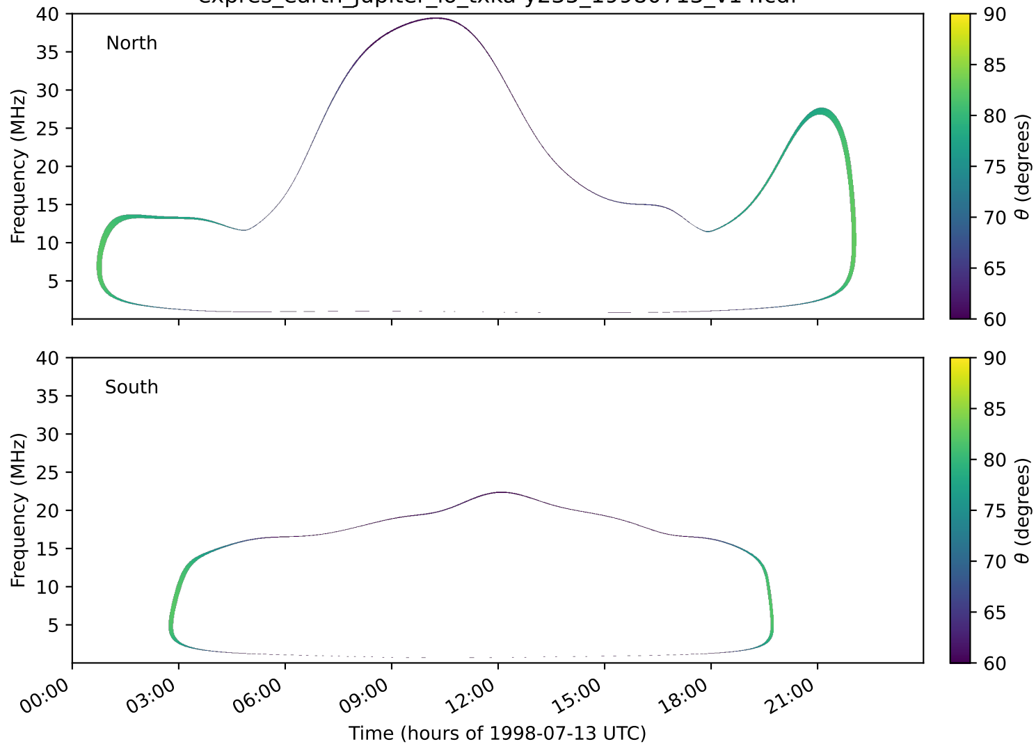
expres_earth_jupiter_io_txka-y235_19980713_v14.cdf
