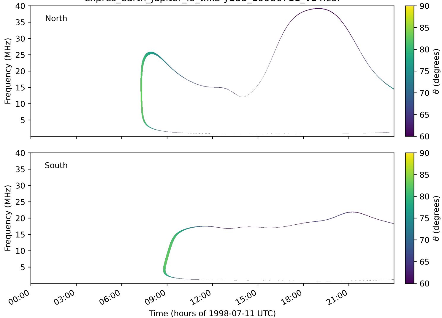
expres_earth_jupiter_io_txka-y235_19980711_v14.cdf
