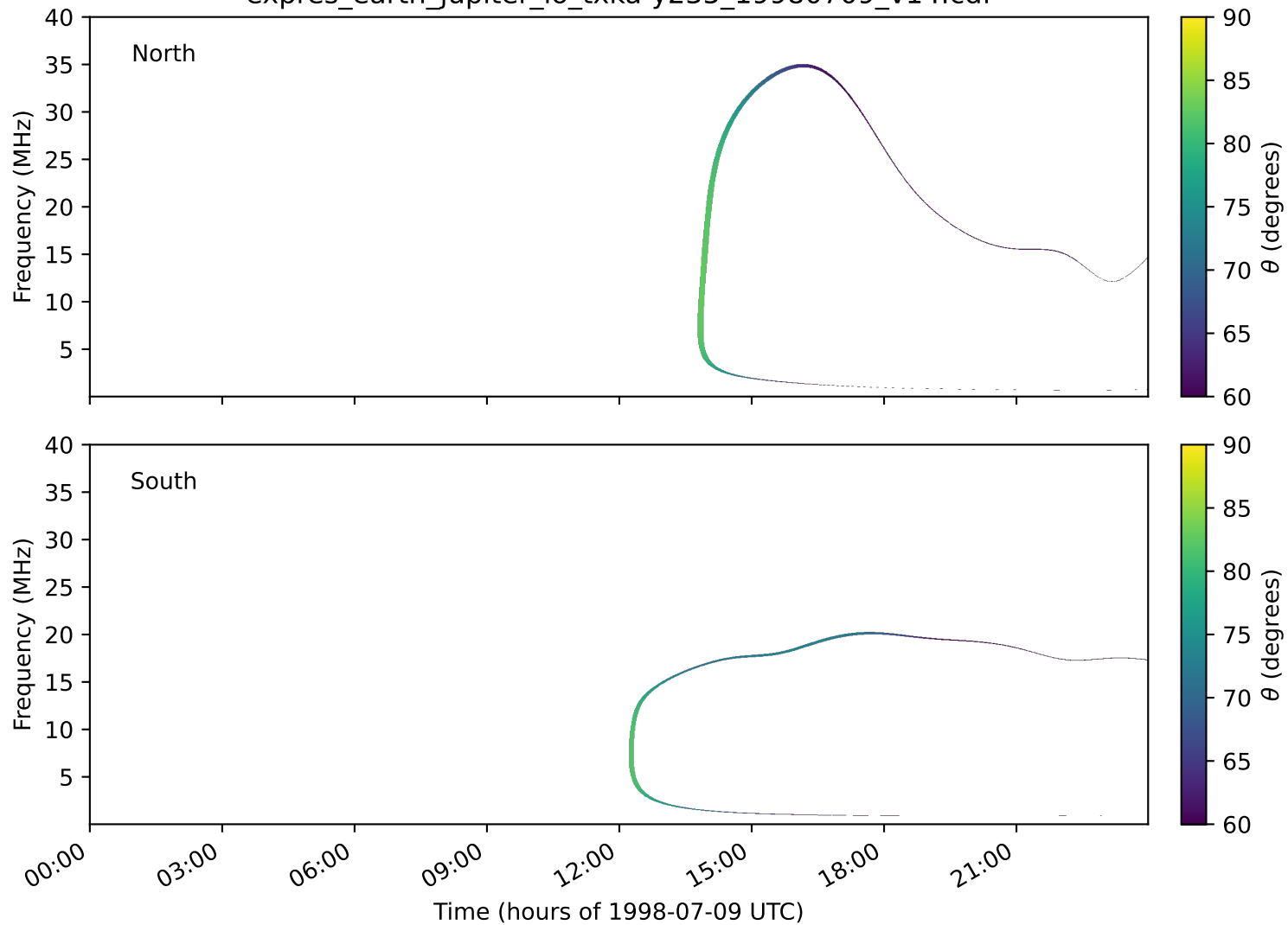
expres_earth_jupiter_io_txka-y235_19980709_v14.cdf
