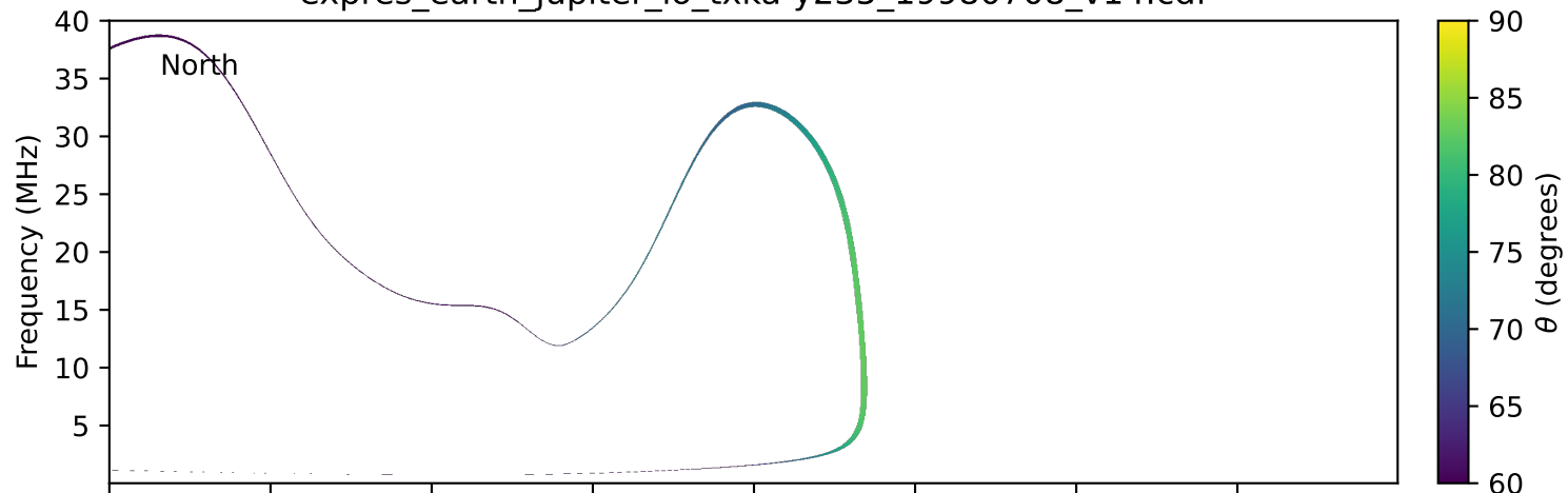
expres_earth_jupiter_io_txka-y235_19980708_v14.cdf
