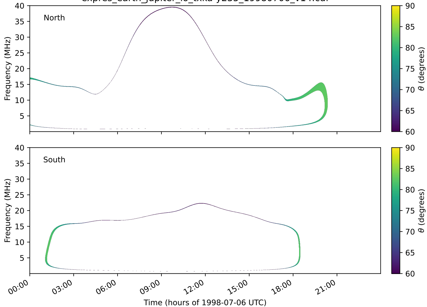
expres_earth_jupiter_io_txka-y235_19980706_v14.cdf
