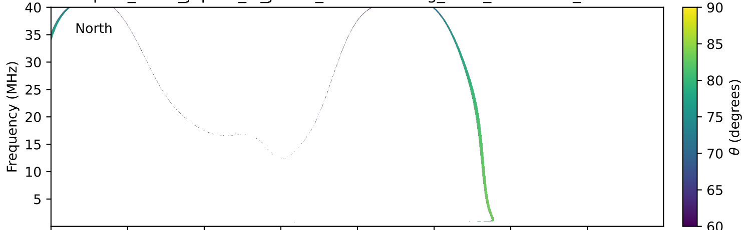
expres_earth_jupiter_io_jrm33_lossc-wid1deg_3kev_19980722_v11.cdf
