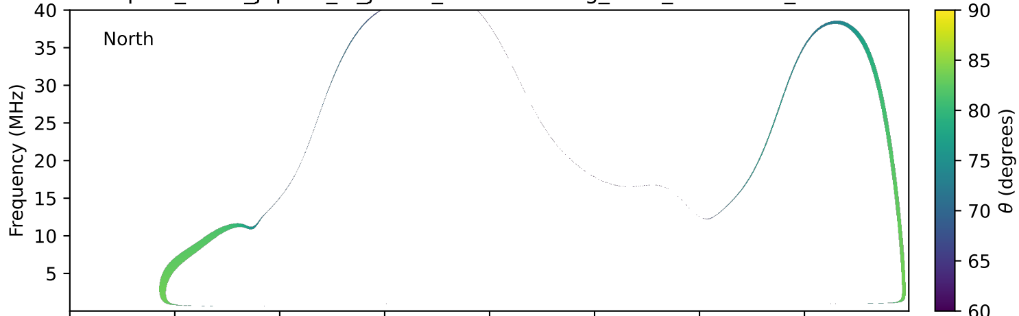
expres_earth_jupiter_io_jrm33_lossc-wid1deg_3kev_19980720_v11.cdf
