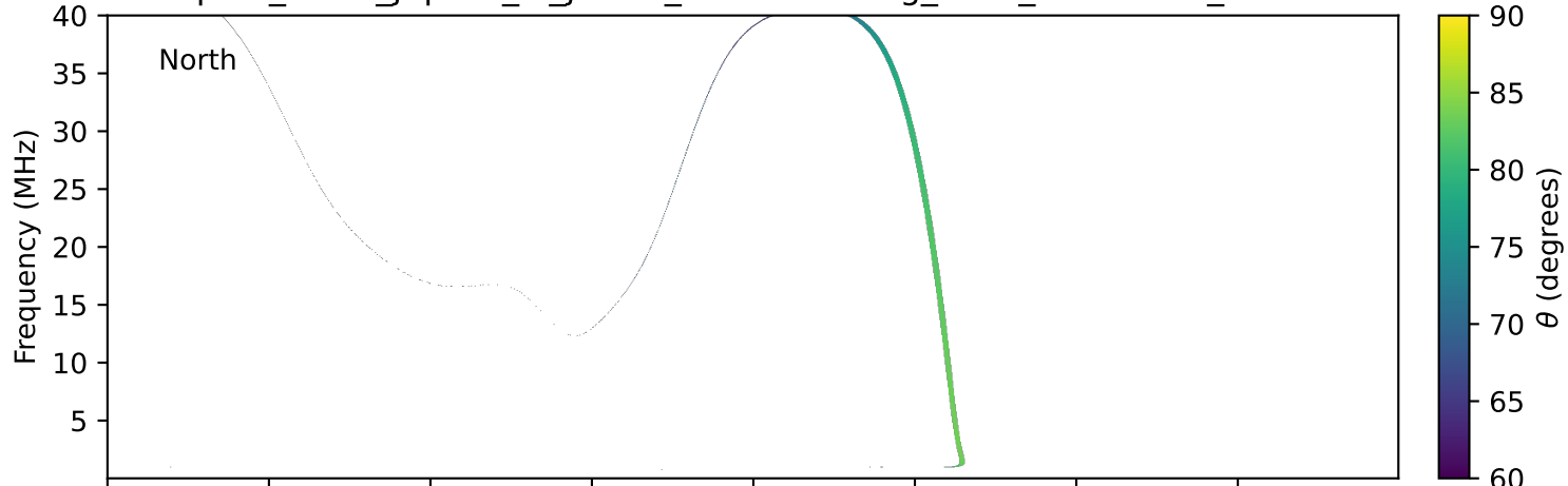
expres_earth_jupiter_io_jrm33_lossc-wid1deg_3kev_19980715_v11.cdf
