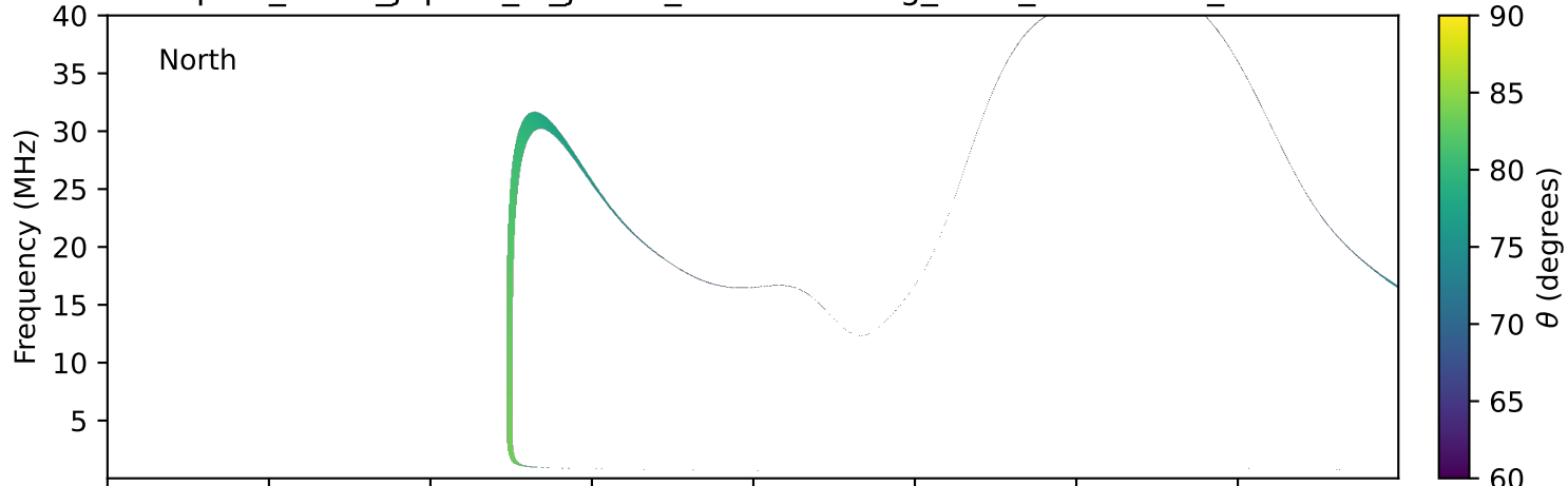
expres_earth_jupiter_io_jrm33_lossc-wid1deg_3kev_19980711_v11.cdf
