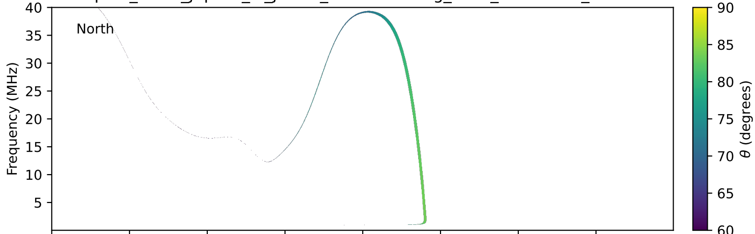
expres_earth_jupiter_io_jrm33_lossc-wid1deg_3kev_19980708_v11.cdf
