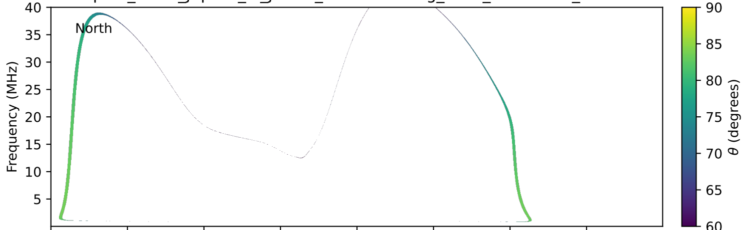
expres_earth_jupiter_io_jrm09_lossc-wid1deg_3kev_19980729_v11.cdf
