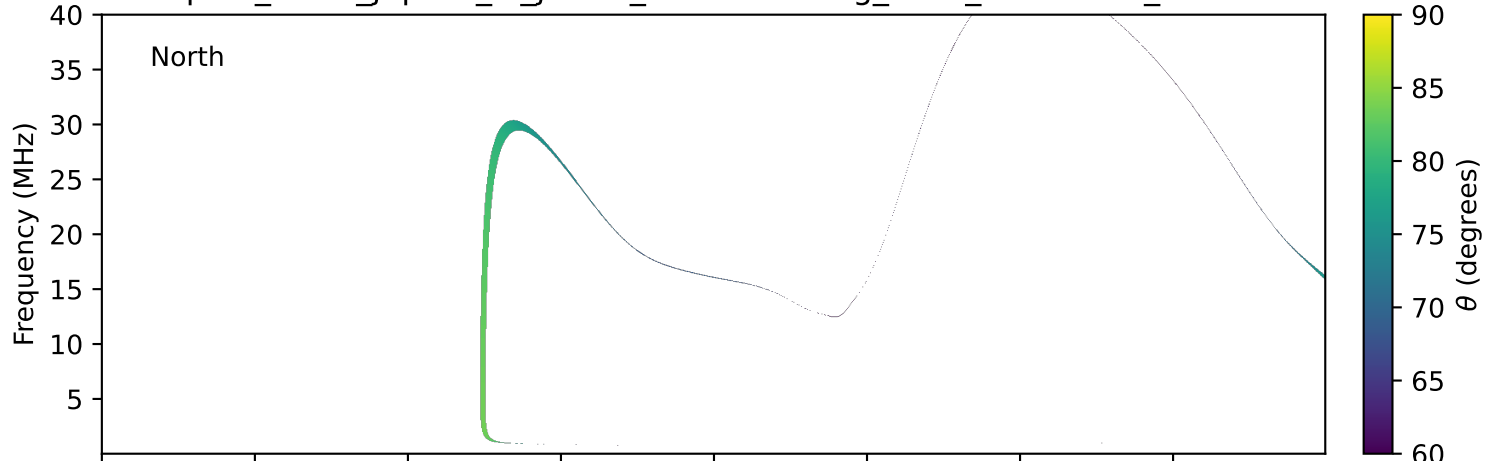
expres_earth_jupiter_io_jrm09_lossc-wid1deg_3kev_19980711_v11.cdf
