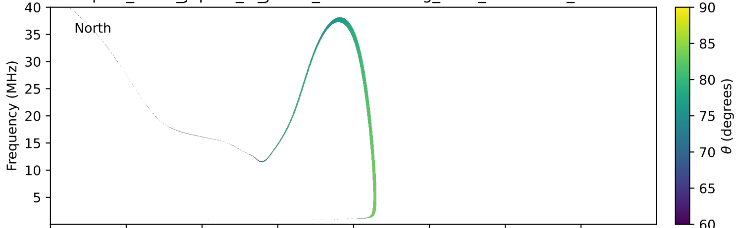
expres_earth_jupiter_io_jrm09_lossc-wid1deg_3kev_19980701_v11.cdf
