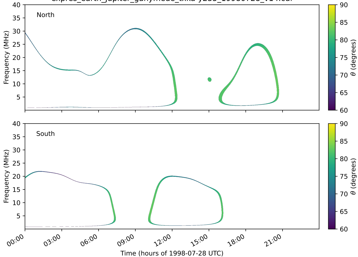
expres_earth_jupiter_ganymede_txka-y235_19980728_v14.cdf
