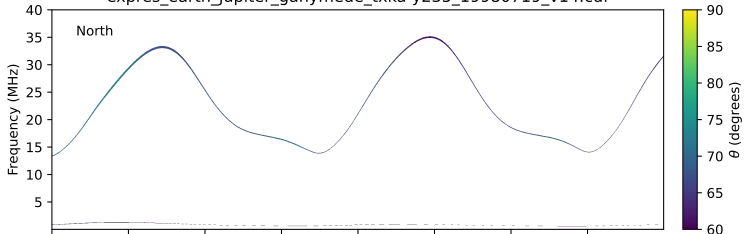
expres_earth_jupiter_ganymede_txka-y235_19980719_v14.cdf
