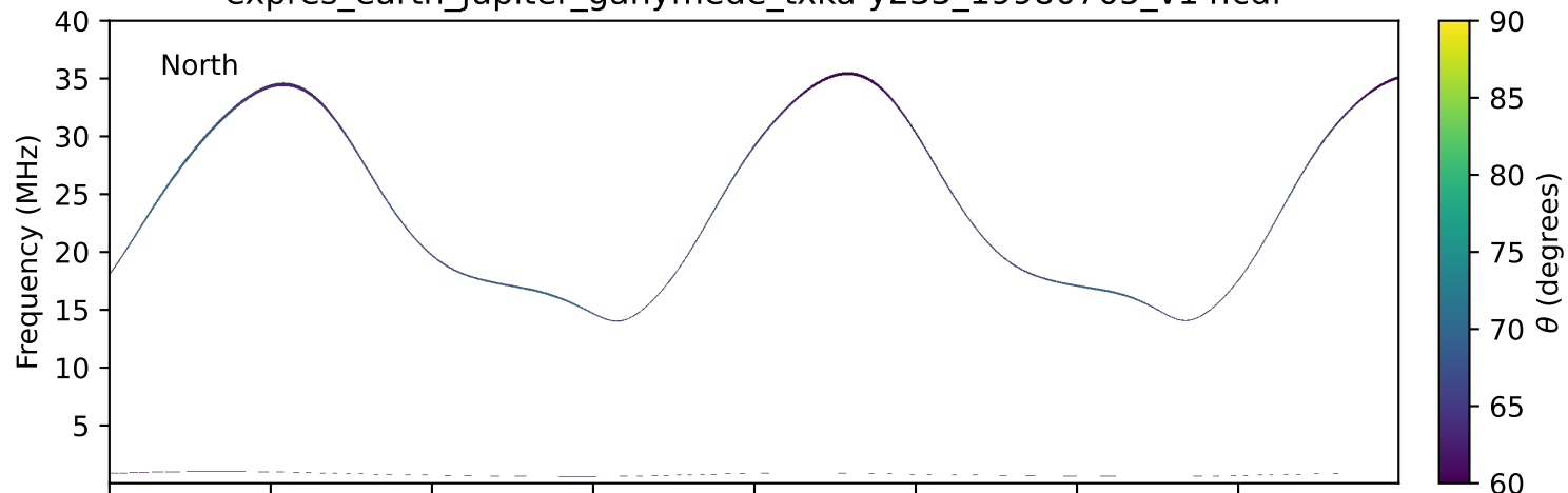
expres_earth_jupiter_ganymede_txka-y235_19980705_v14.cdf
