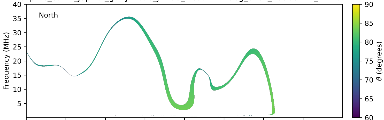
expres_earth_jupiter_ganymede_jrm33_lossc-wid1deg_3kev_19980714_v11.cdf
