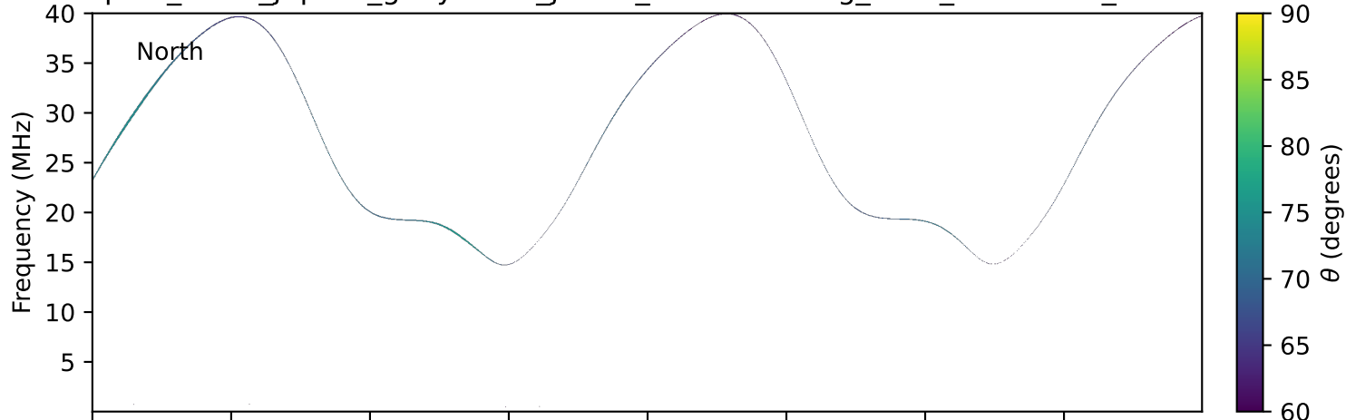
expres_earth_jupiter_ganymede_jrm33_lossc-wid1deg_3kev_19980705_v11.cdf
