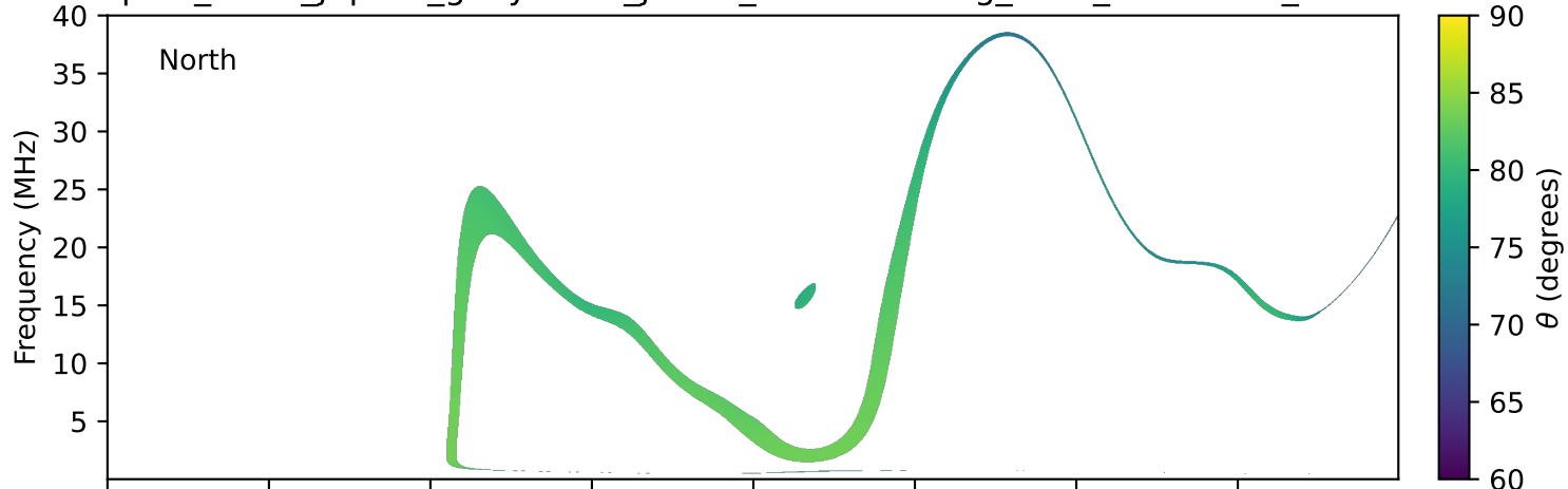
expres_earth_jupiter_ganymede_jrm33_lossc-wid1deg_3kev_19980704_v11.cdf
