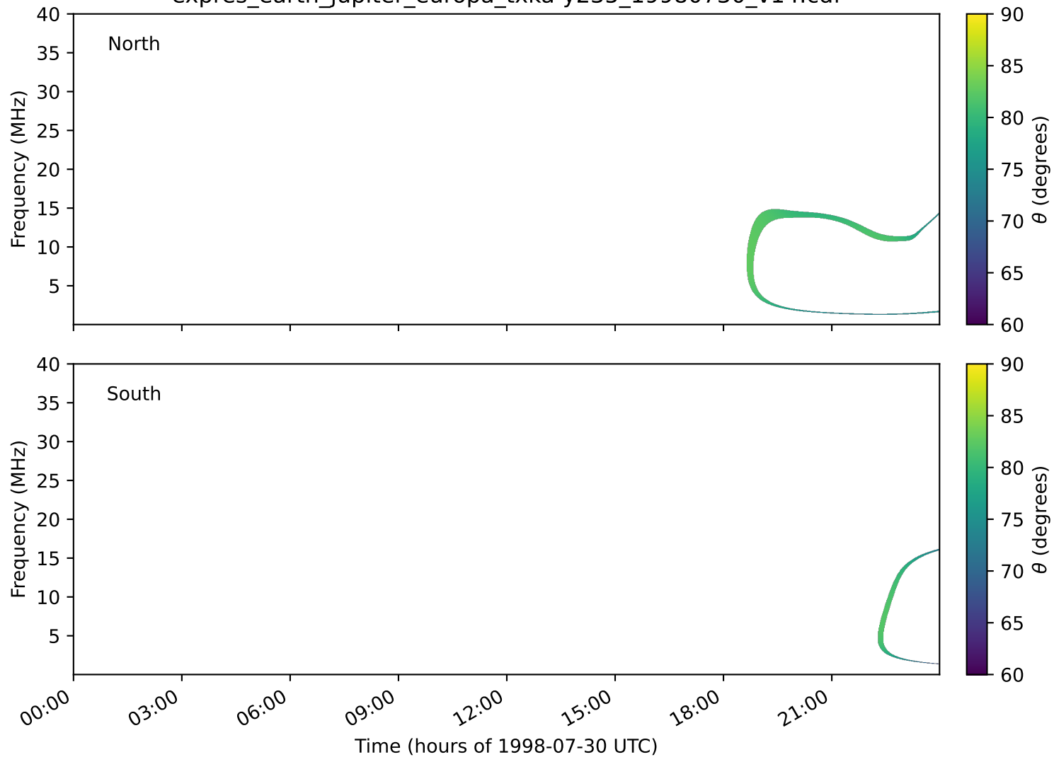
expres_earth_jupiter_europa_txka-y235_19980730_v14.cdf
