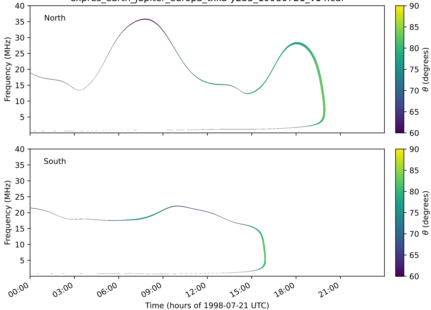
expres_earth_jupiter_europa_txka-y235_19980721_v14.cdf
