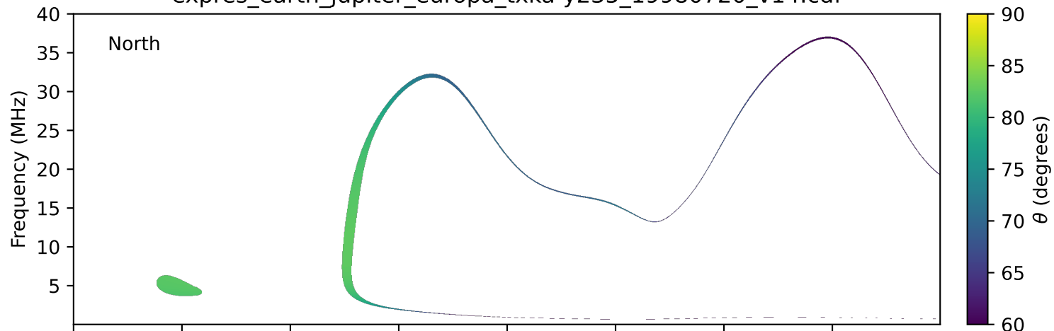
expres_earth_jupiter_europa_txka-y235_19980720_v14.cdf
